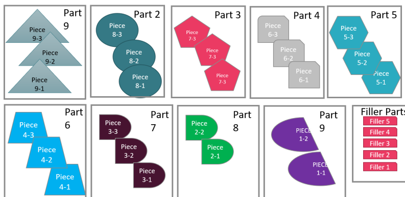
Figure 2: Simple nesting for composite part manufacturing. The unused white space in each index represents composite material that will be discarded. In some of the indexes, 50% of the material available is not being used.
